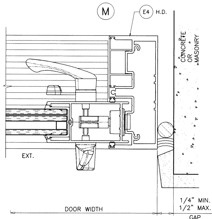
FREE STANDING H. DUTY JAMB OPERABLE SIDE
