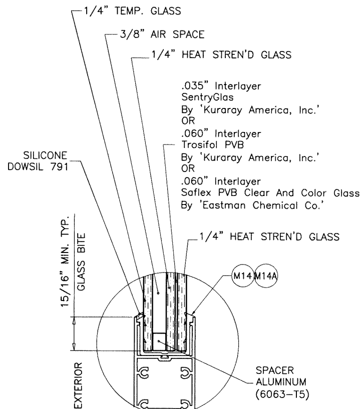
GLASS TYPE 'CI'
