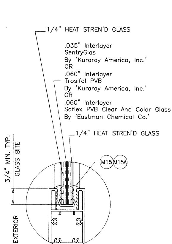
GLASS TYPE 'C'
