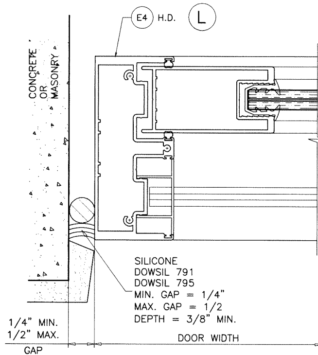
FREE STANDING H. DUTY JAMB FIXED SIDE
